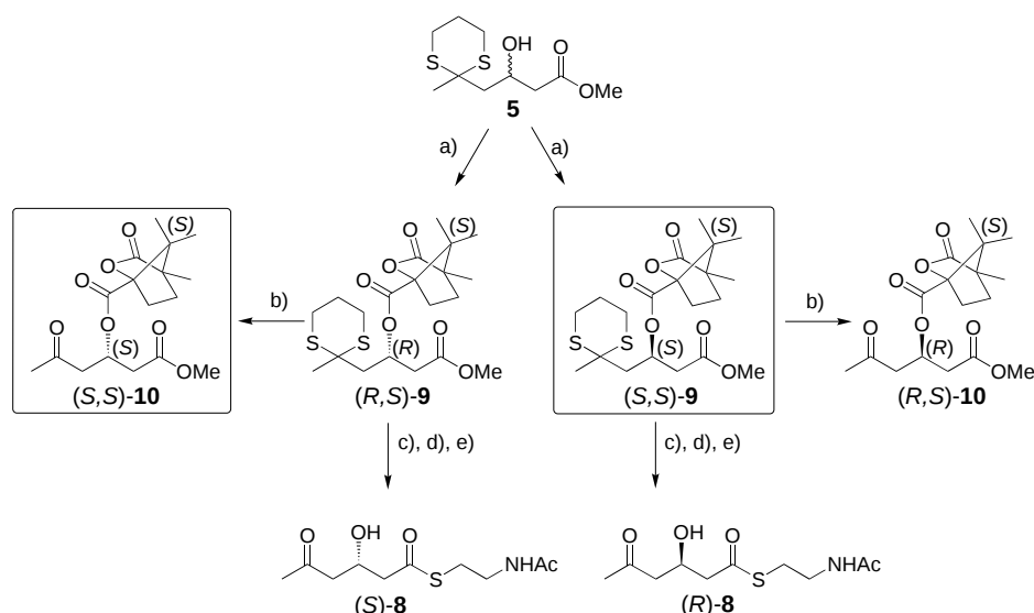
Scheme 3. Reagents and conditions: a) ( S )-camphanoyl chloride, \text{NEt}_3 , DMAP, 1,2-dichloroethane (DCE), b) \text{Me}_3\text{O}^+\text{BF}_4^- , dichloromethane (DCM), c) 3.5 M HCl/2 M NaOH, HCl, d) (\text{PhO})_2\text{P}(\text{O})(\text{N}_3) , N -acetylcysteamine, DMF, e) MeI, \text{CaCO}_3 , 50 °C [8] . The boxed structures have been determined by X-ray crystallography.
